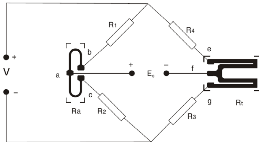
Figure 4: Zero balance compensation
