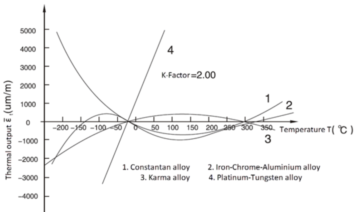
Figure 1: Thermal output curve of strain gauges on different steel materials
