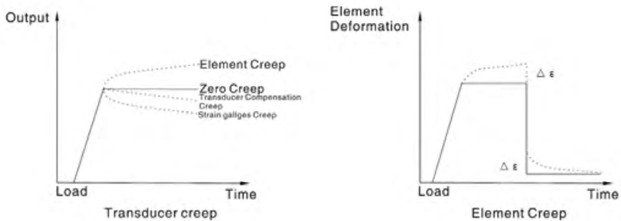
Figure 3: Creep compensation and effect of creep
