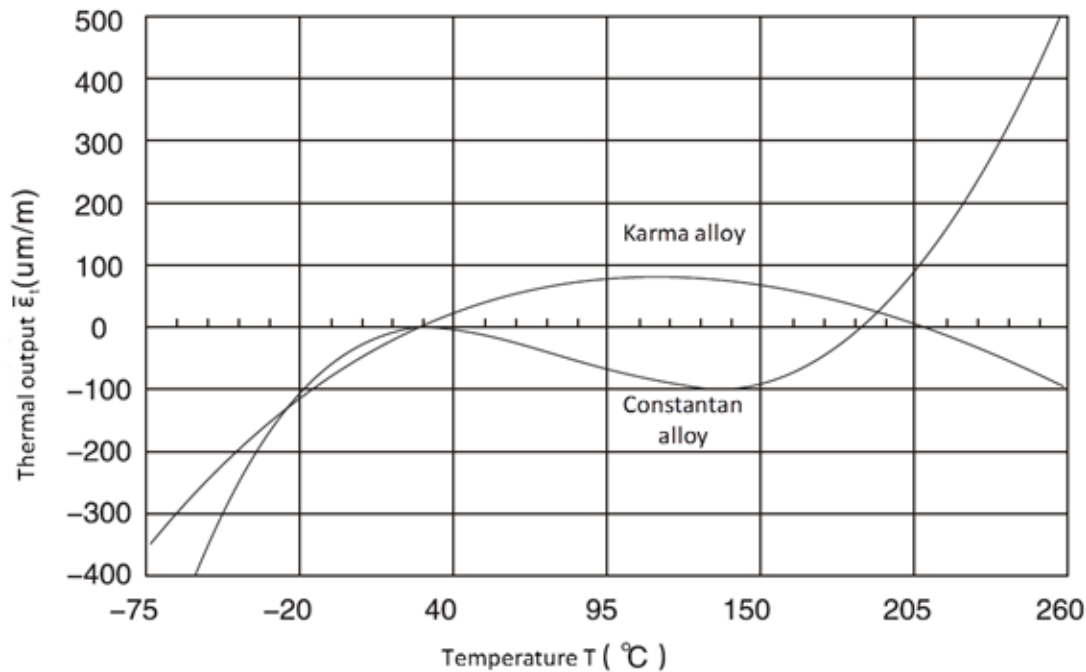
Figure 2: Thermal output for Self-Temperature compensated Karma and Constantan alloy strain gauges
