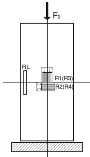
Figure 6: Semi-conductor bonding location
