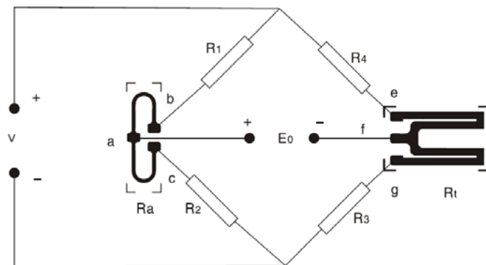
Figure 5: Zero temperature compensation
