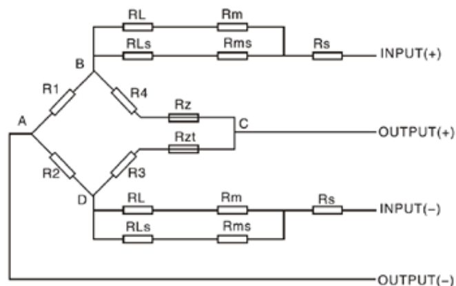
Figure 7: Linear compensations location in a full bridge sketch
